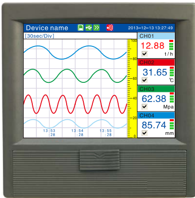
Timing curves (lengthways) Measured values, channel number, engineering unit, alarm status and accumulative message,all of them will be displayed in timing curves.
