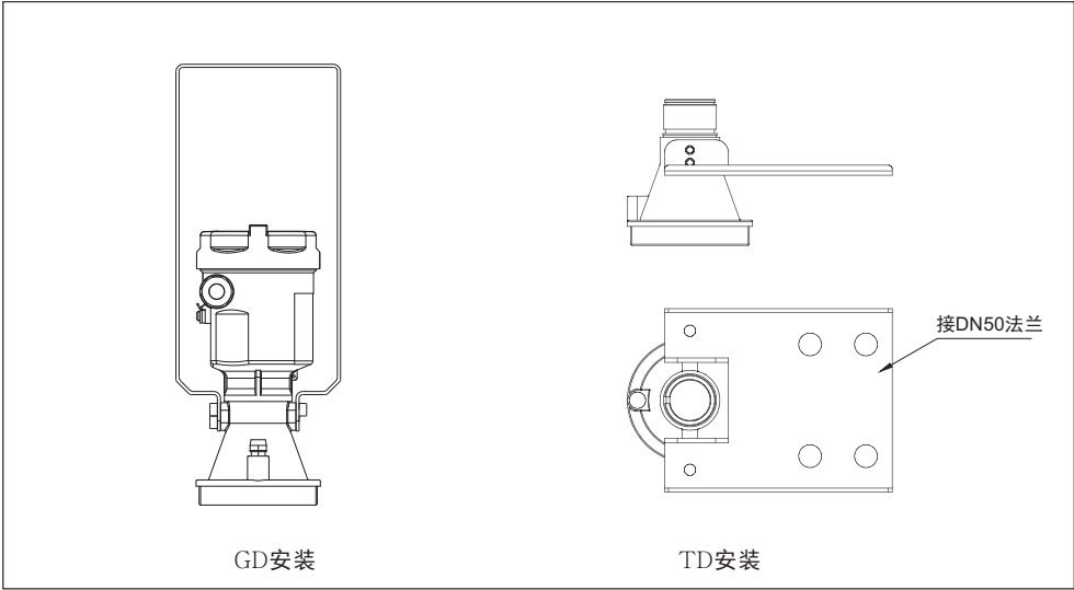
SDRD81/87 Antenna:GD/TD
