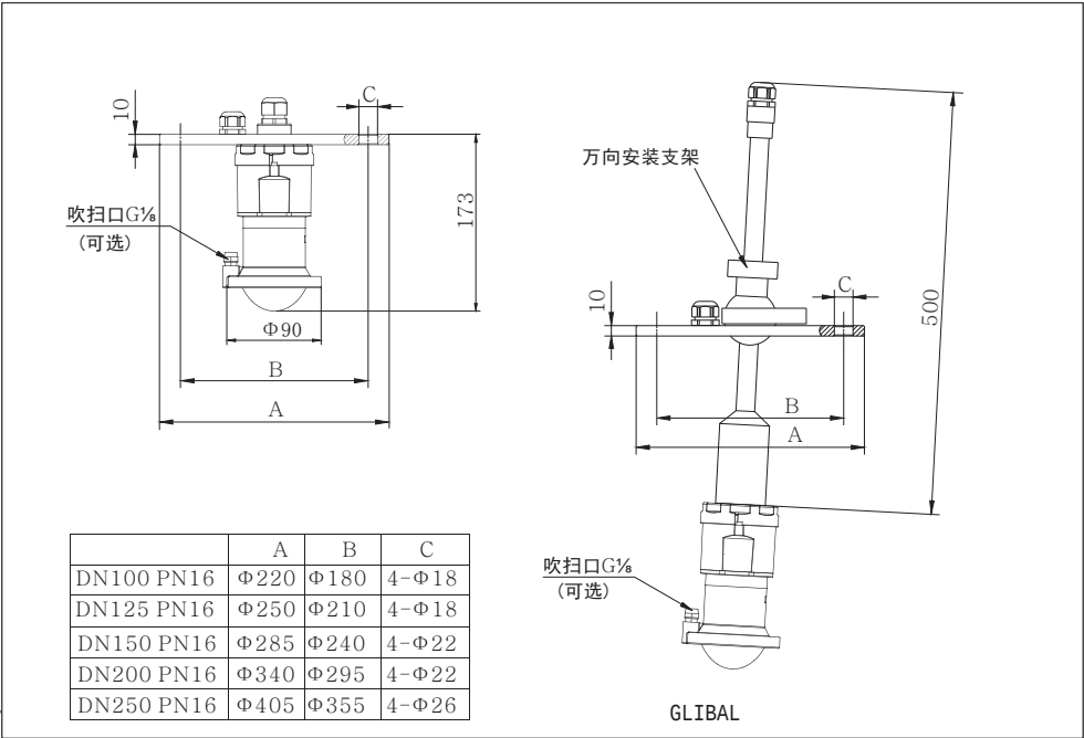
SDRD 88 Install
